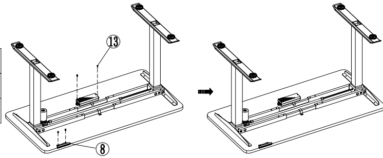
Connection diagram
